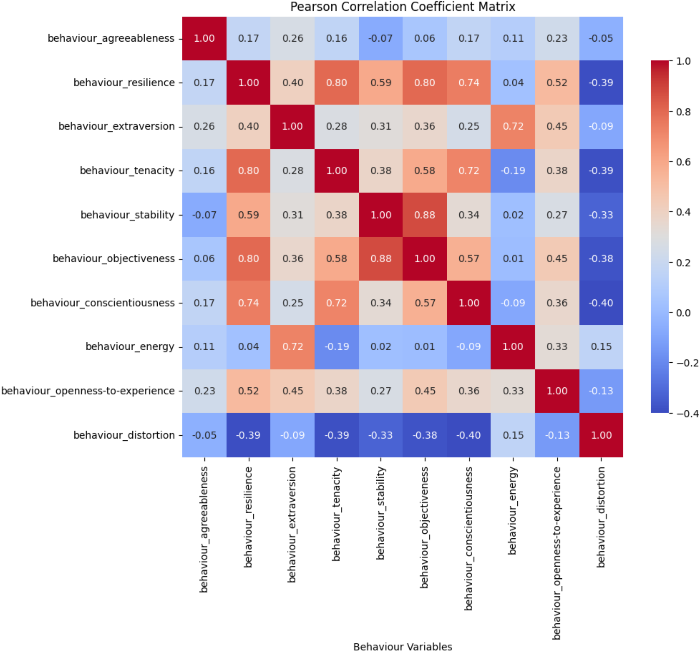
Behaviour Variables
